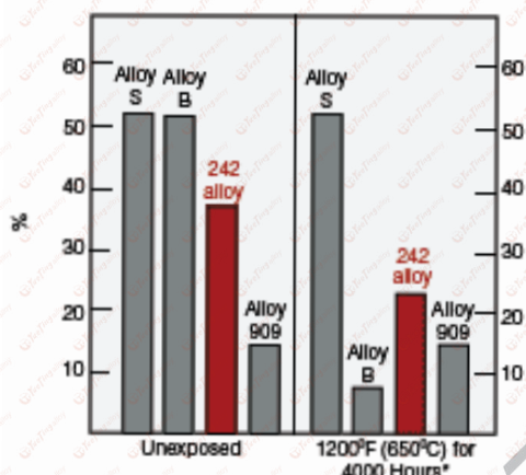
Room-Temperature Tensile Elongation
